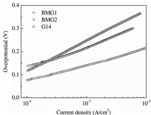
Fig. 5. Tafel plots of BMG1, BMG2 and G14 after pretreatment using 1 M HF solution for 1 min.
