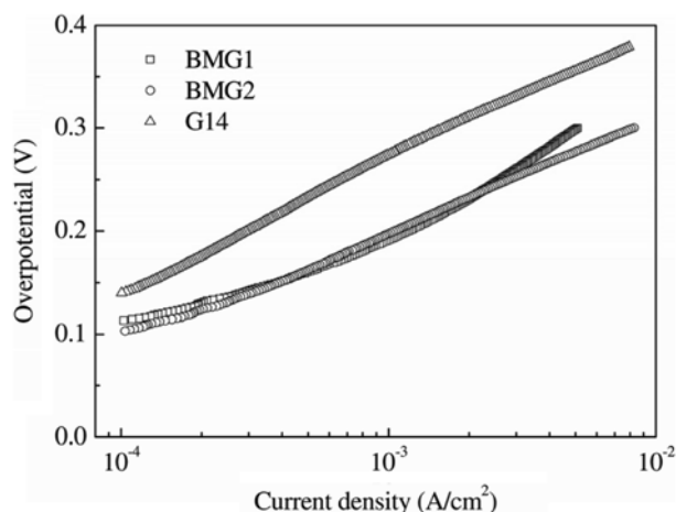
Fig. 4. Tafel plots of BMG1, BMG2 and G14 at as-cast state.
